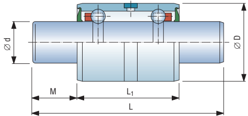
Type: 型号: 76-3-1
