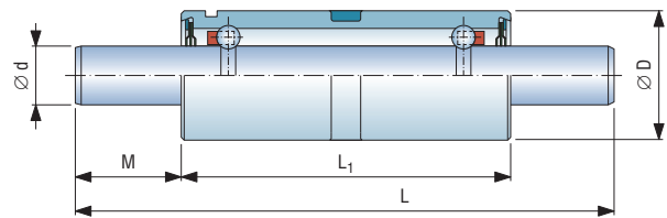
Type: 型号: 73-1-14, 73-1-20, 73-1-22
