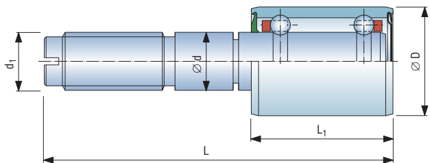
Type: 型号: 76-3-1
