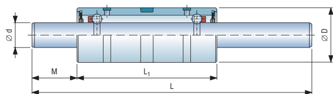
Type: 型号: 73-1-14, 73-1-20, 73-1-22
